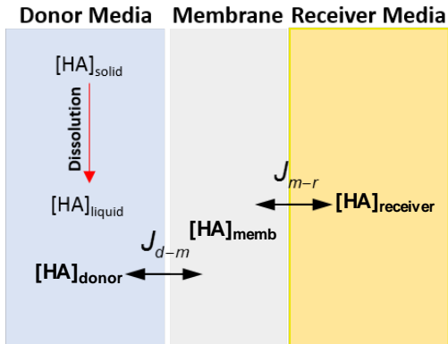
Mathematical model of a Transwell.
