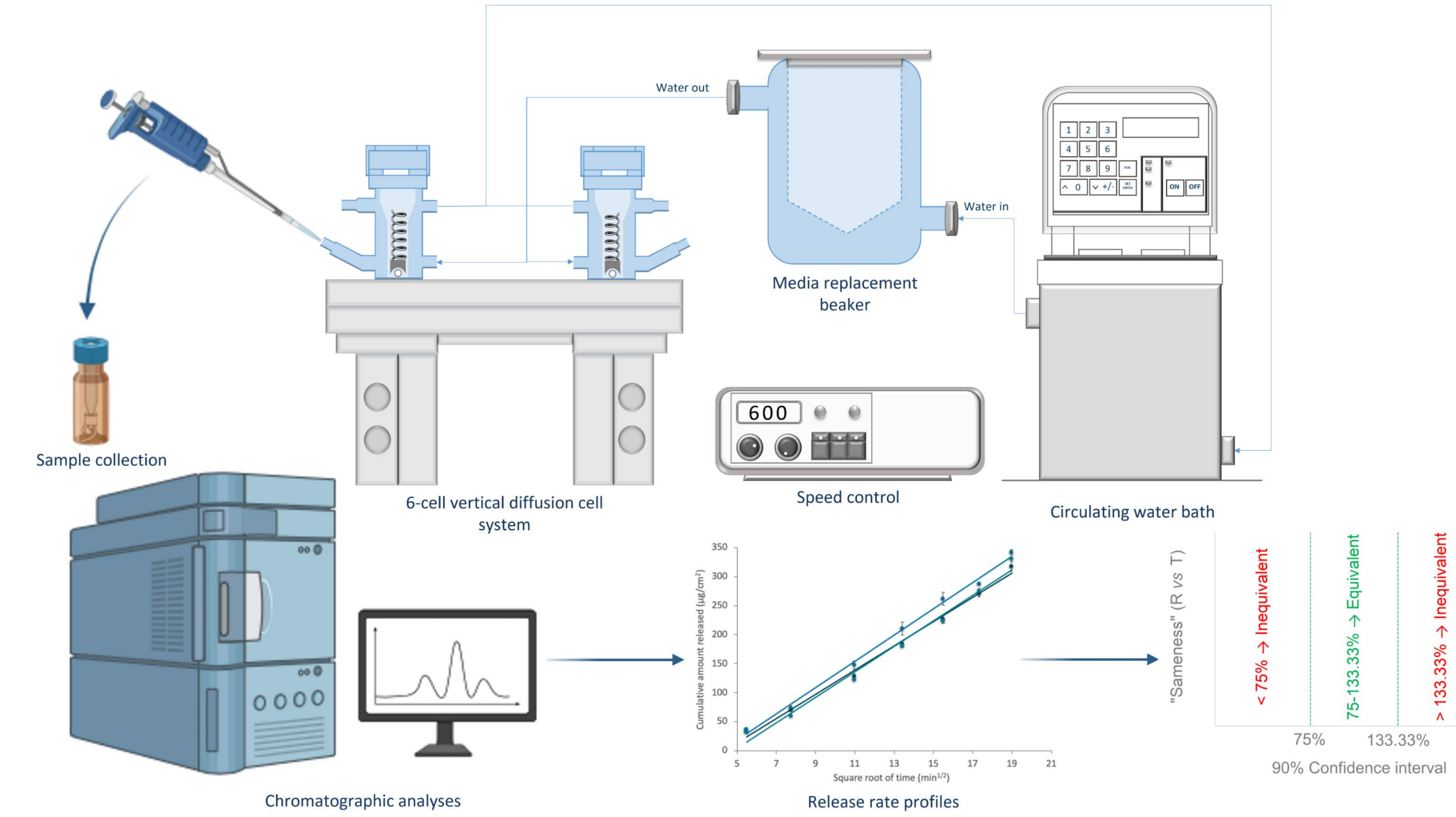
Figure 2. Schematic representation of the IVRT methodology
