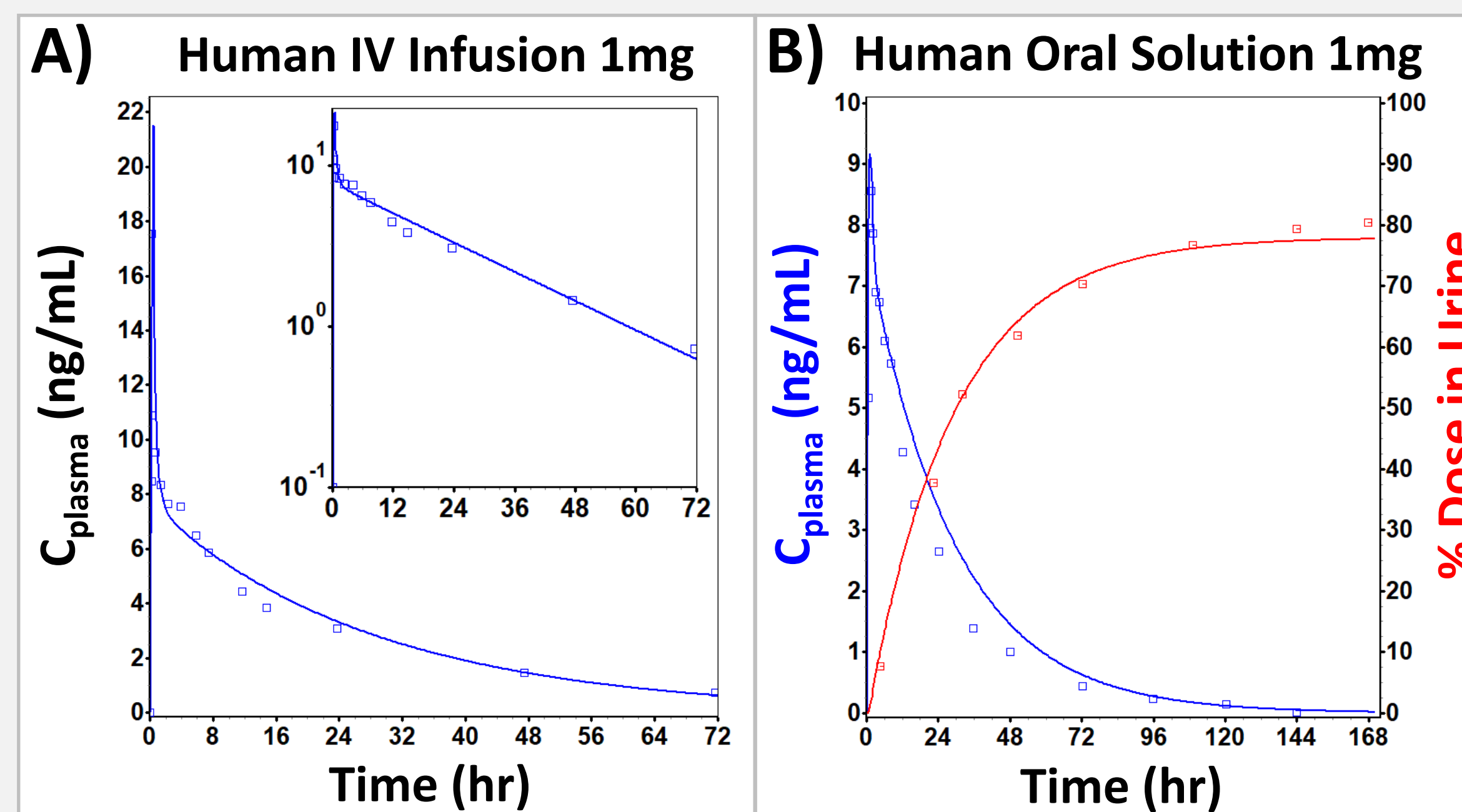
Figure 2: Observed vs. predicted plasma concentration vs. time for (A) 1 mg IV infusion of paliperidone and (B) 1 mg oral solution of paliperidone.
