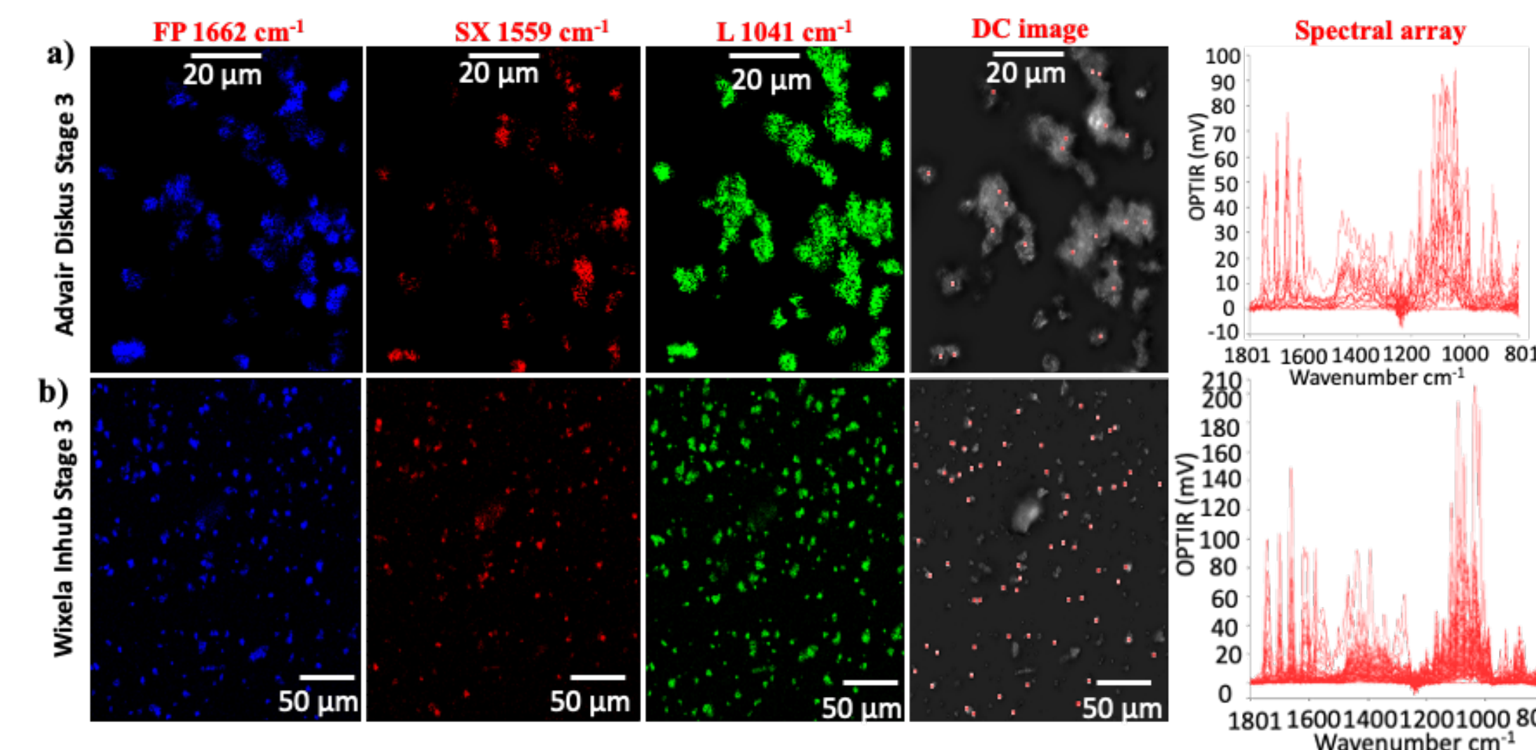
Single wavenumber chemical maps, direct current (DC) image and spectral array collected from aerosolised a) Advair Diskus 100/50 and b) Wixela Inhub 100/50 particles collected from Stage 3 of the NGI showing the distribution of FP, SX, and L.
