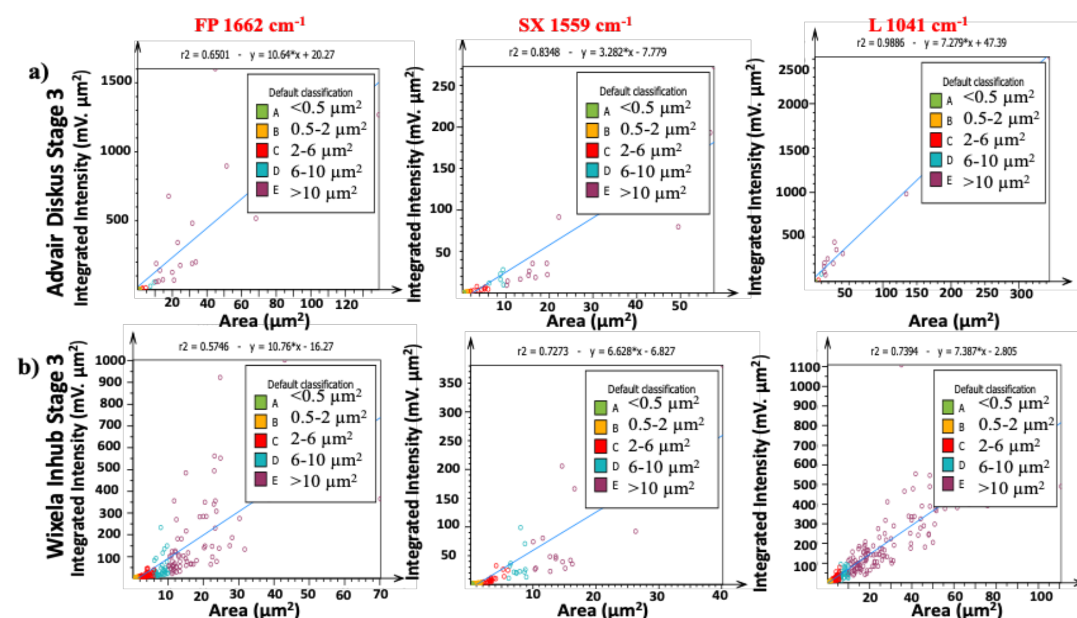
Scattered plots of integrated intensity vs. area of particles demonstrating the particle size distribution of FP, SX, and L across the aerosolised a) Advair Diskus 100/50 and b) Wixela Inhub 100/50 particles collected from Stage 3 of the NGI.
