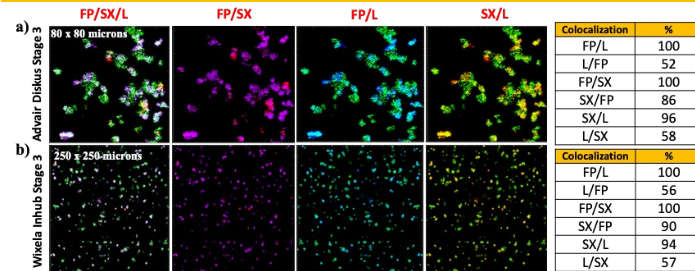
Colocalization analysis of FP, SX, and L of aerosolised a) Advair Diskus 100/50 and b) Wixela Inhub 100/50 particles collected from Stage 3 of the NGI. Degree of colocalization is represented as a percentage (%) via the Manders Coefficient.
