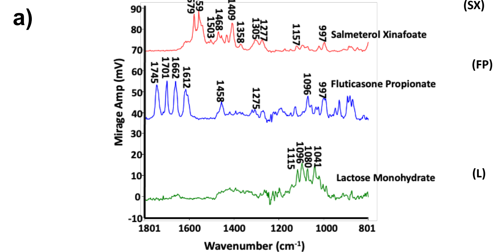
a) O-PTIR spectra of fluticasone propionate (FP), salmeterol xinafoate (SX), and lactose (L) raw materials. Representative identification peaks are labelled for each component.
