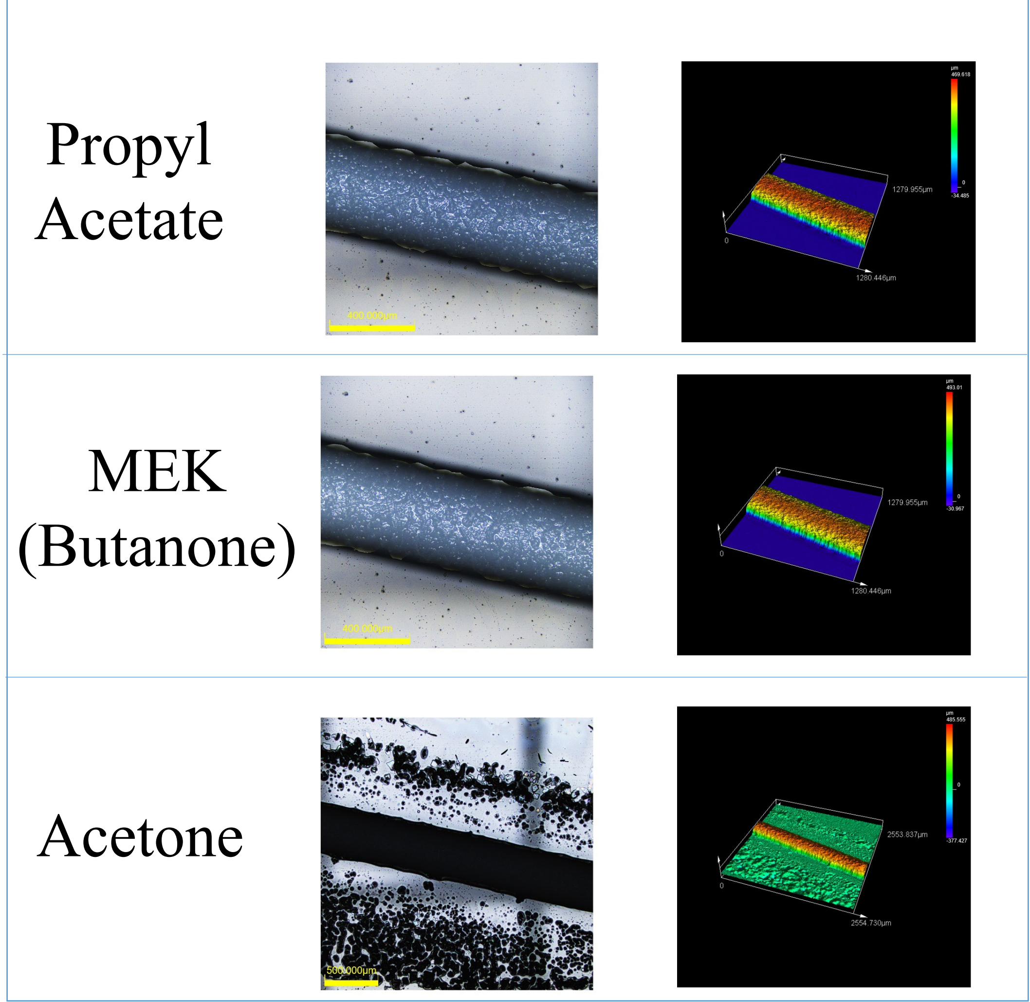
Figure 1. Confocal images collected at indicated solvent vapor conditions. All solvents collected at 10X magnification except for acetone which was collected at 5X. Display shows both color image (left) and color-coded height image (right).
